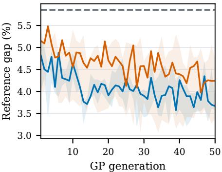
AS
